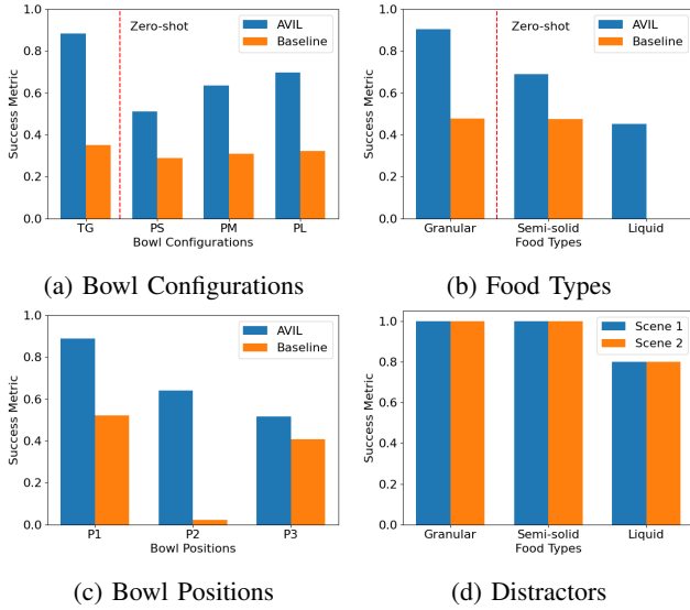
Fig. 3: Experimental results. (a-c) Performance comparison between AVIL and baseline across varied bowl configurations, food types and bowl positions. We present on the right side of the dashed red line in (a-b) conditions tested zero-shot. (d) AVIL performance with and without distractors. Scene 1 represents without distractors and Scene 2 represents with distractors.
