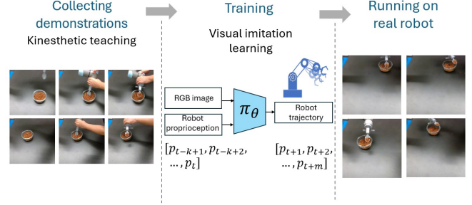
Fig. 1: Learning pipeline diagram of our approach (AVIL) for spoon scooping in RAF.
