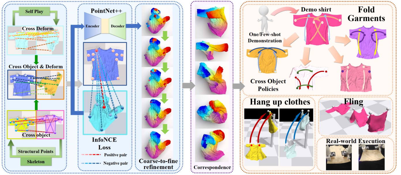
Fig. 2: Our Proposed Learning Framework for Dense Visual Correspondence. (Left) We extract the cross-deform correspondence and cross-object correspondence point pairs respectively using self-play and skeletons, and train the per-point correspondence scores in the contrastive manner, with the Coarse-to-fine module refines the quality. (Middle) Learned correspondence demonstrates point-level similarity across different garments in different deformations. (Right) The learned point-level correspondence can facilitates multiple diverse downstream tasks using one or few-shot demonstrations.
